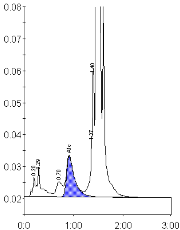
Peak table - ID: 10420079
