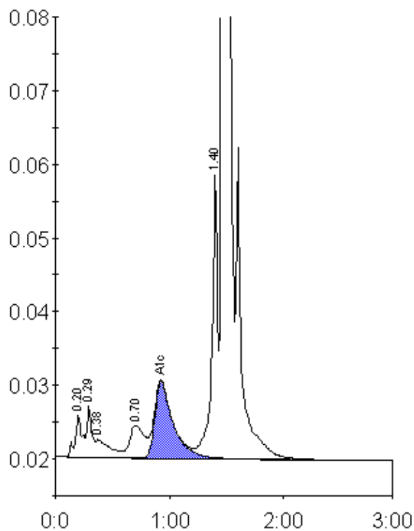
Peak table - ID: 10547361
